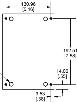
BOTTOM VIEW OF ENCLOSURE
