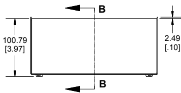
BACK VIEW OF ENCLOSURE
