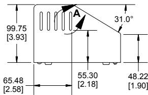
END VIEW OF ENCLOSURE
