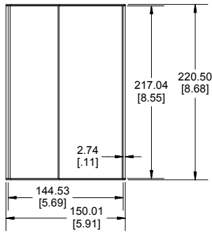
TOP VIEW OF ENCLOSURE
