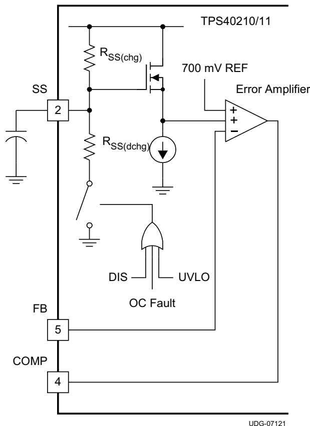
Figure 21. SS Pin Functional Circuit
