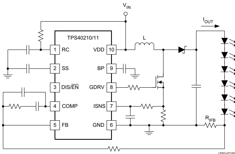
Figure 29. Typical LED Drive Schematic
