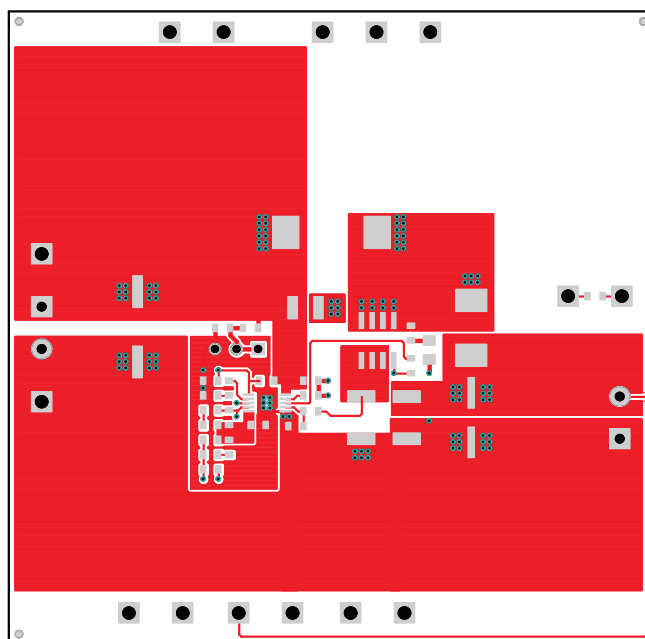
Figure 38. Top Copper
