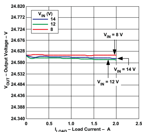
Figure 35. Output Voltage vs Load Current
