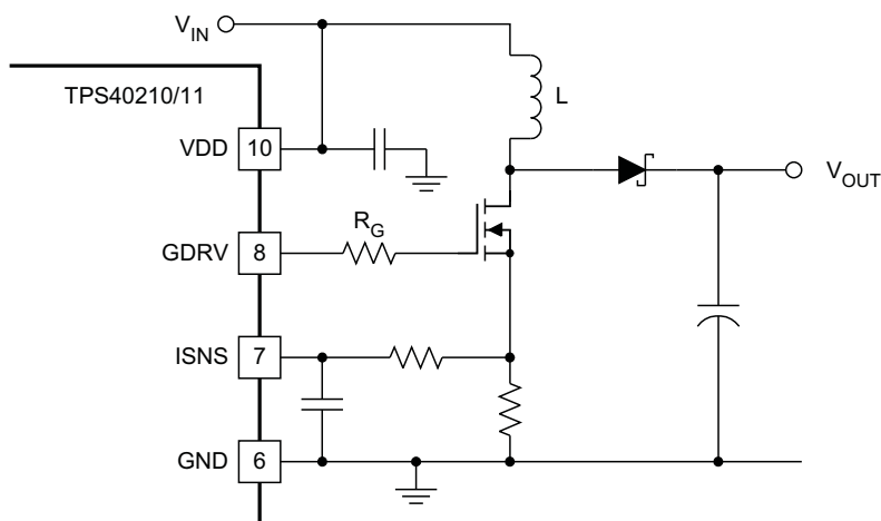
Figure 28. Gate Drive Resistor
