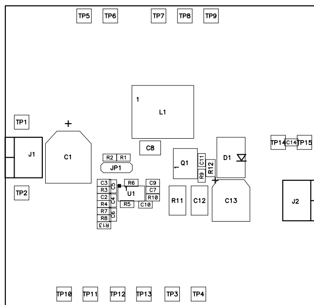
Figure 37. Component Placement
