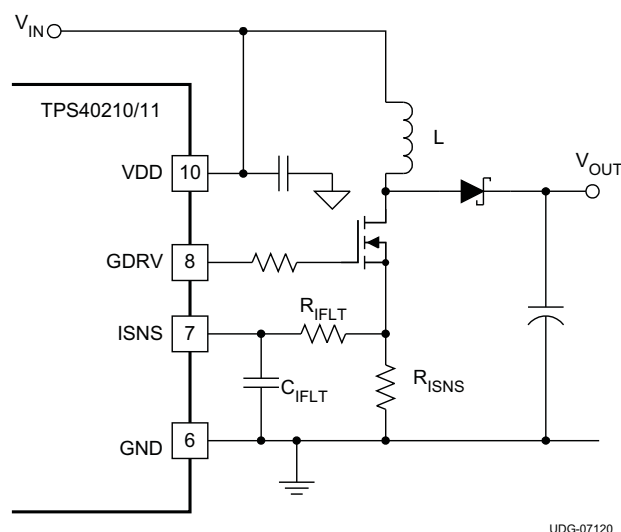
Figure 26. Current Sense Components
