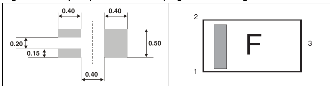
Figure 10. Footprint (dimensions in mm) Figure 11. Marking
