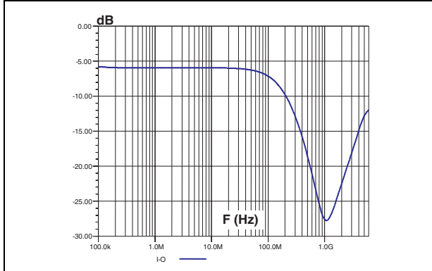
Figure 4. S21 attenuation measurement (V bias = 0 V)
