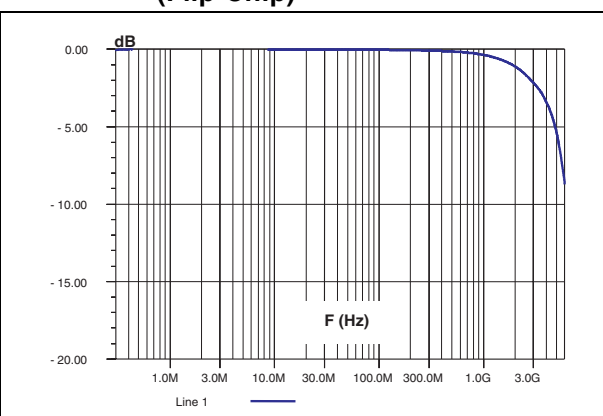
Figure 18. S21 attenuation measurement results of channel 1 (Flip-Chip)
