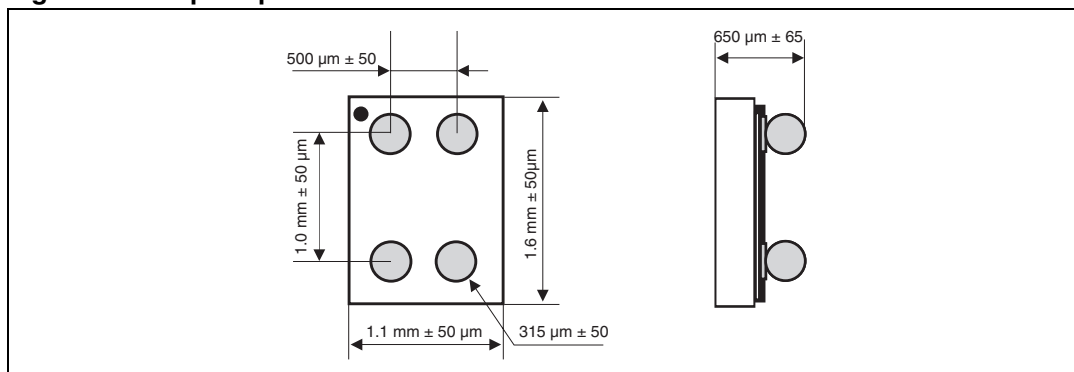
Figure 25. Flip-Chip dimensions
