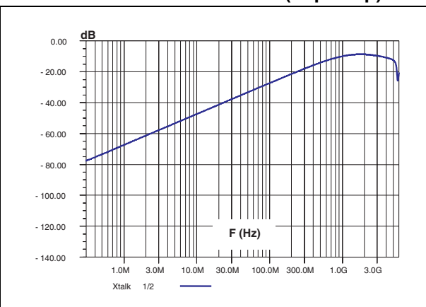
Figure 20. Analog crosstalk measurements between channels (Flip-Chip)
