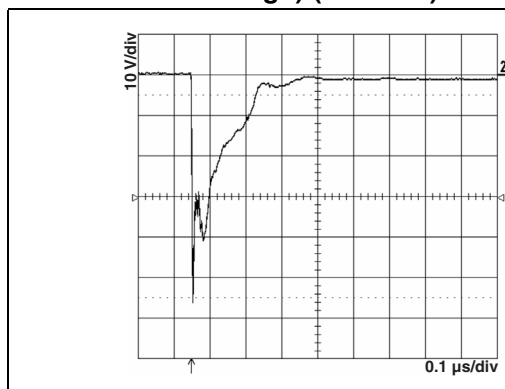
Figure 15. Remaining voltage after ESDAULC6-3BP6 during ESD 15 kV negative surge (air discharge) (SOT-666)
