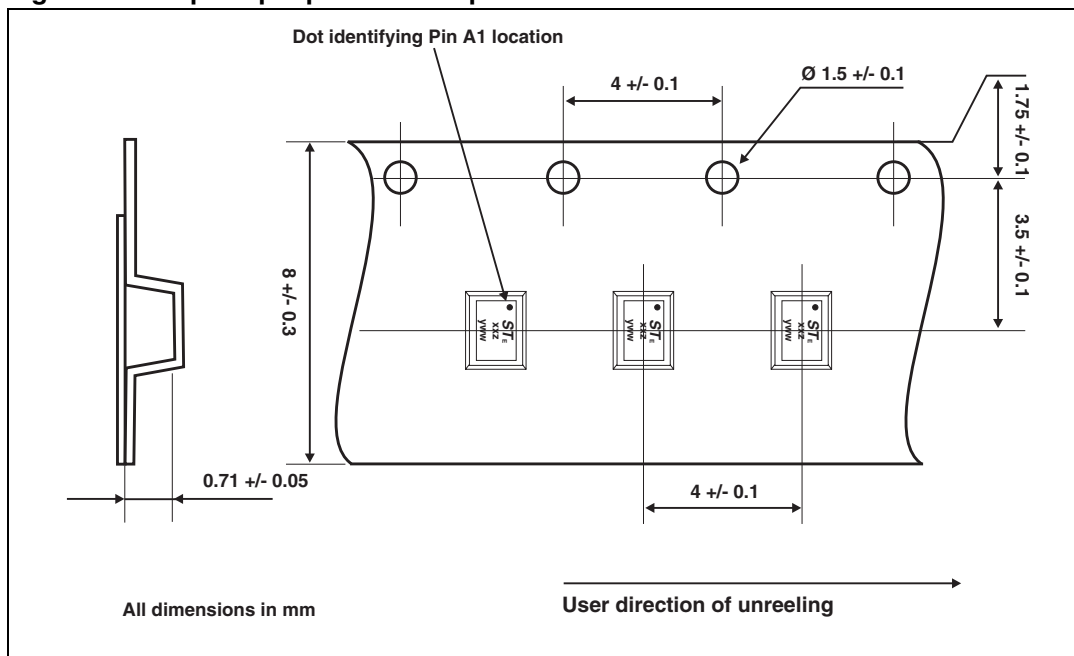
Figure 28. Flip-Chip tape and reel specifications
