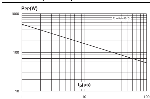
Figure 5. Peak pulse power versus exponential pulse duration (SOT-666)
