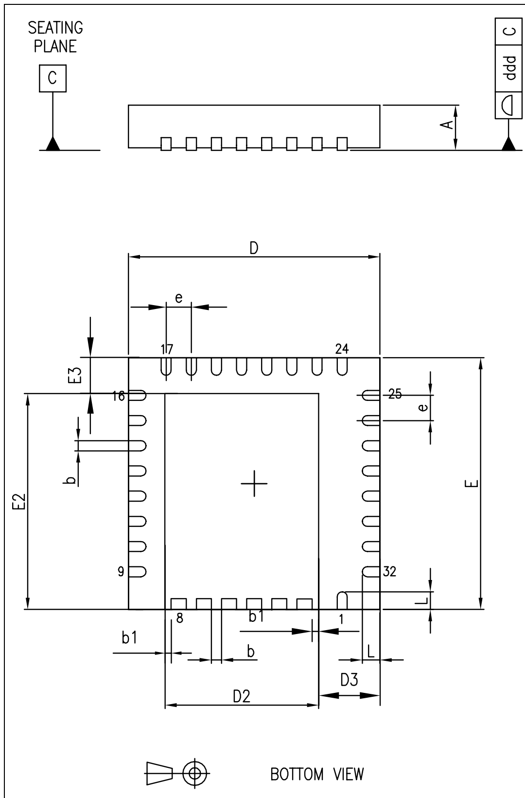
Figure 20. Package dimensions
