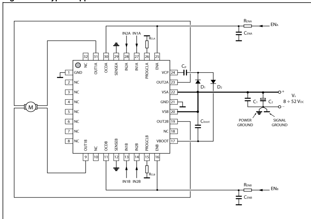
Figure 14. Typical application
