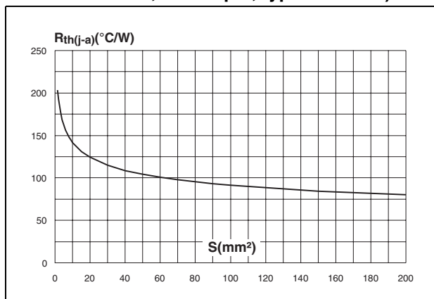
Figure 11. Thermal resistance junction to ambient versus copper surface under tab (epoxy printed board FR4, Cu=35 µm, typical values)
