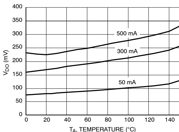
Figure 11. Dropout Voltage vs. Temperature 2.8 V Version
