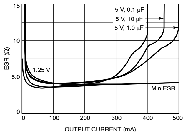
Figure 27. Output Current vs. ESR
