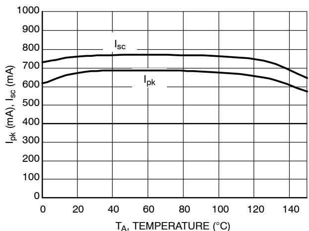
Figure 15. Peak and Short Current vs. Temperature
