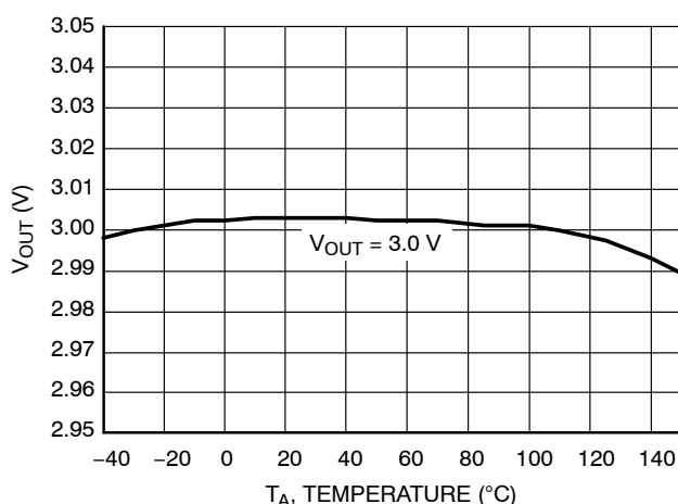
Figure 6. Output Voltage vs. Temperature 3.0 V Version
