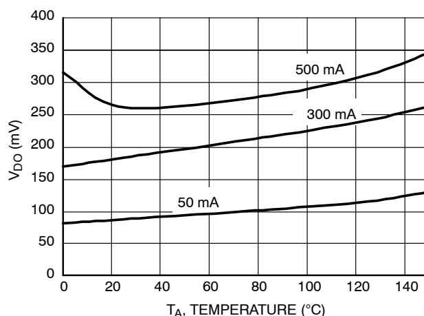
Figure 12. Dropout Voltage vs. Temperature 2.5 V Version
