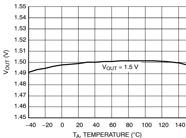
Figure 10. Output Voltage vs. Temperature 1.5 V Version
