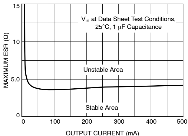
Figure 26. Stability with ESR vs. I_{out}
