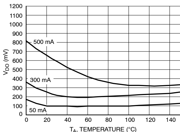
Figure 13. Dropout Voltage vs. Temperature 1.8 V Version
