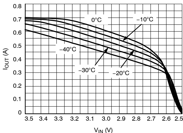
Figure 20. Output Current Capability for the 2.5 V Version
