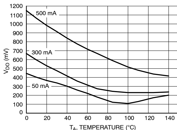
Figure 14. Dropout Voltage vs. Temperature 1.5 V Version
