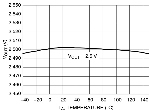
Figure 8. Output Voltage vs. Temperature 2.5 V Version
