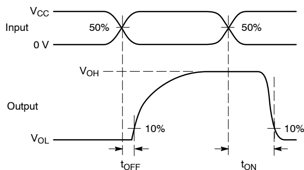
Figure 9. t_{ON}/t_{OFF}
