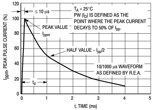
Figure 2. Pulse Waveform
