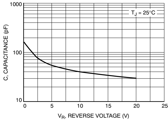
Figure 17. Capacitance
