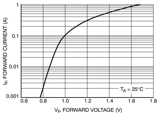
Figure 4. Forward Voltage
