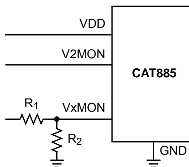
Figure 1. CAT885 Programming Trip Voltage
