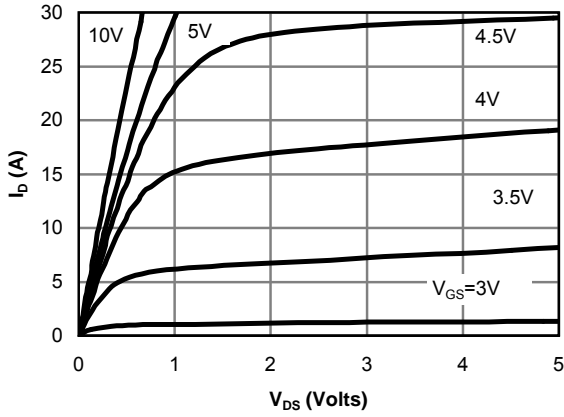
Fig 1: On-Region Characteristics
