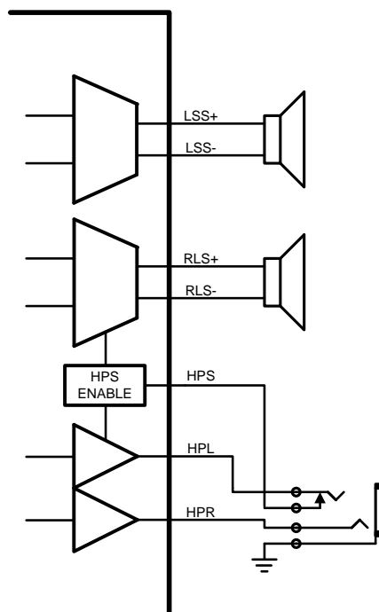
Figure 71. HPS Connection
