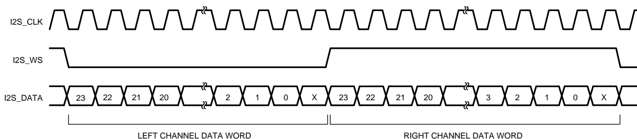
Figure 69. I 2 S Left-Justified Input Format
