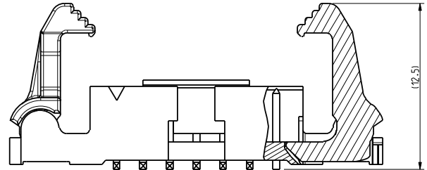
EXAMPLE 10078995-G02-14YLF LOW PROFILE LATCH
