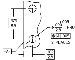
MOUNTING HOLE PATTERN
