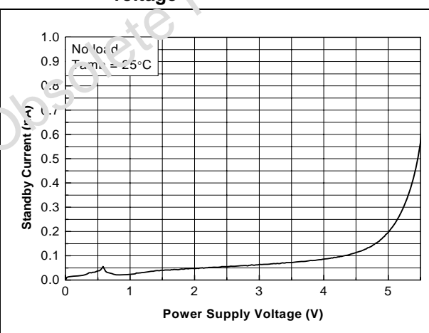
Figure 53. Standby current vs. power supply voltage
