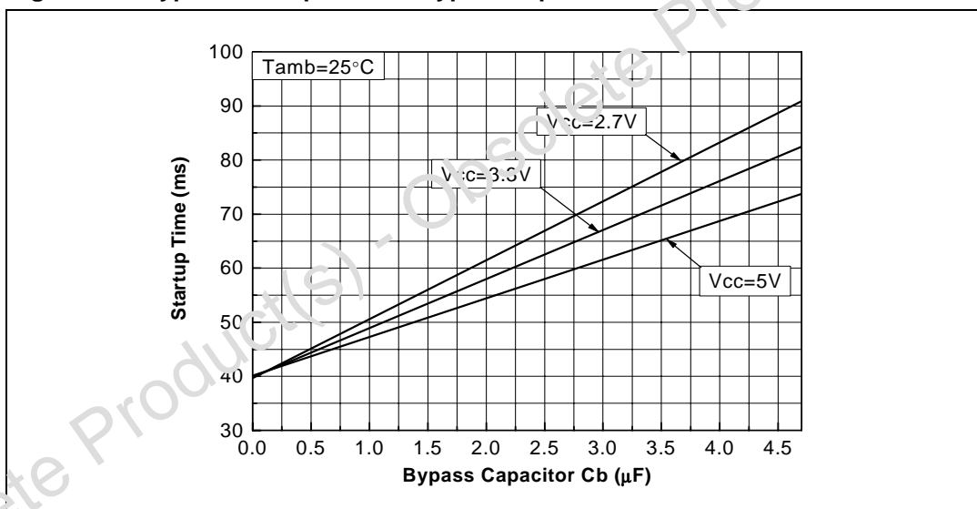
Figure 66. Typical startup time vs. bypass capacitor
