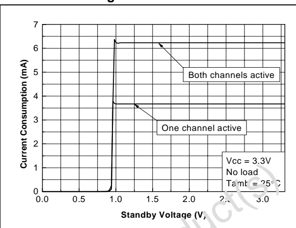
Figure 51. Current consumption vs. standby voltage
