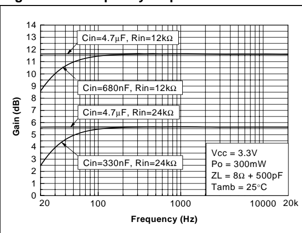
Figure 55. Frequency response
