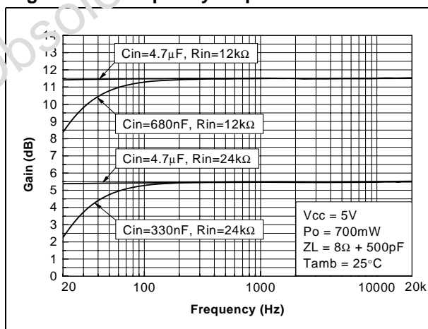
Figure 54. Frequency response
