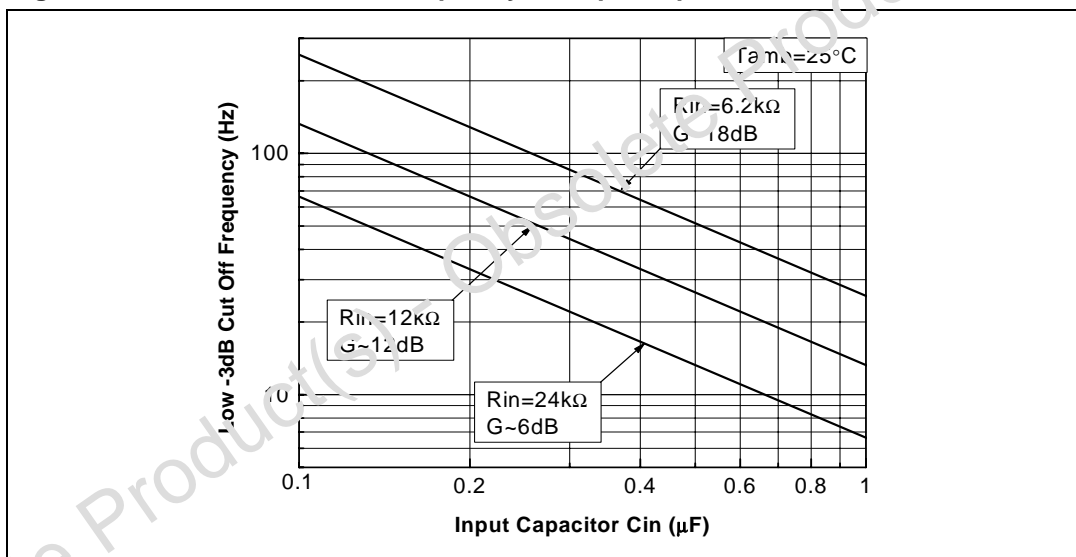
Figure 64. -3dB lower cut-off frequency vs. input capacitance
