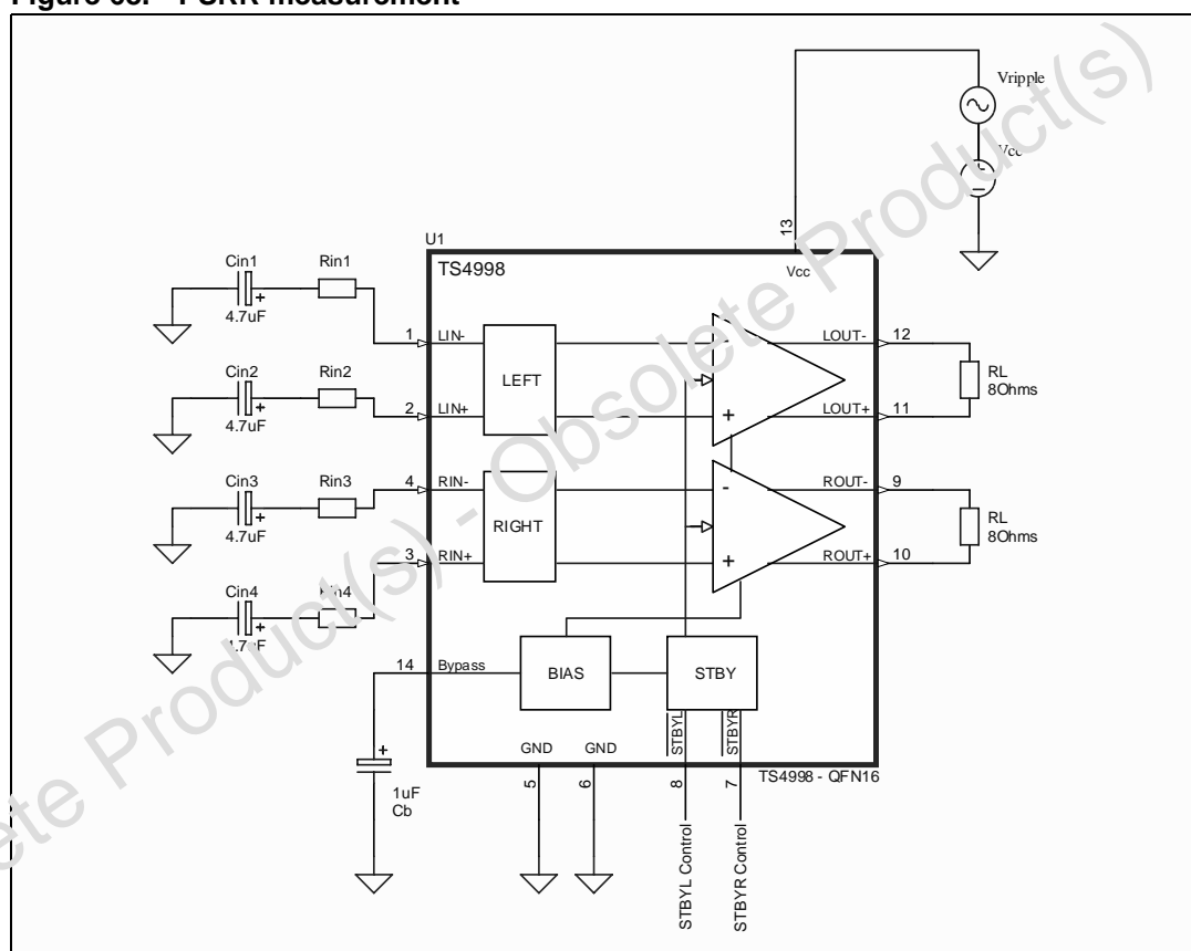
Figure 68. PSRR measurement
