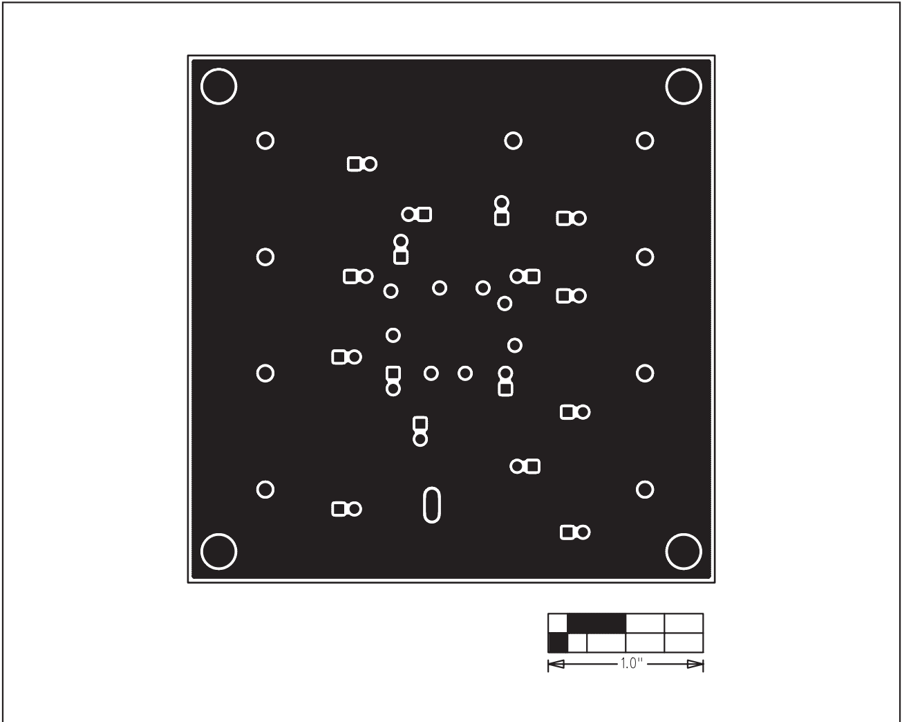
Figure 4. MAX11504 EV Kit PCB Layout—Solder Side
