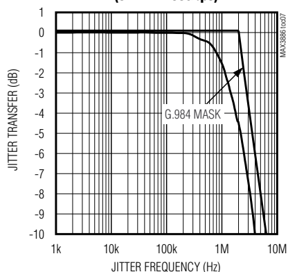
SDI TO SDO JITTER TRANSFER (SDI = 2.488Gbps)
