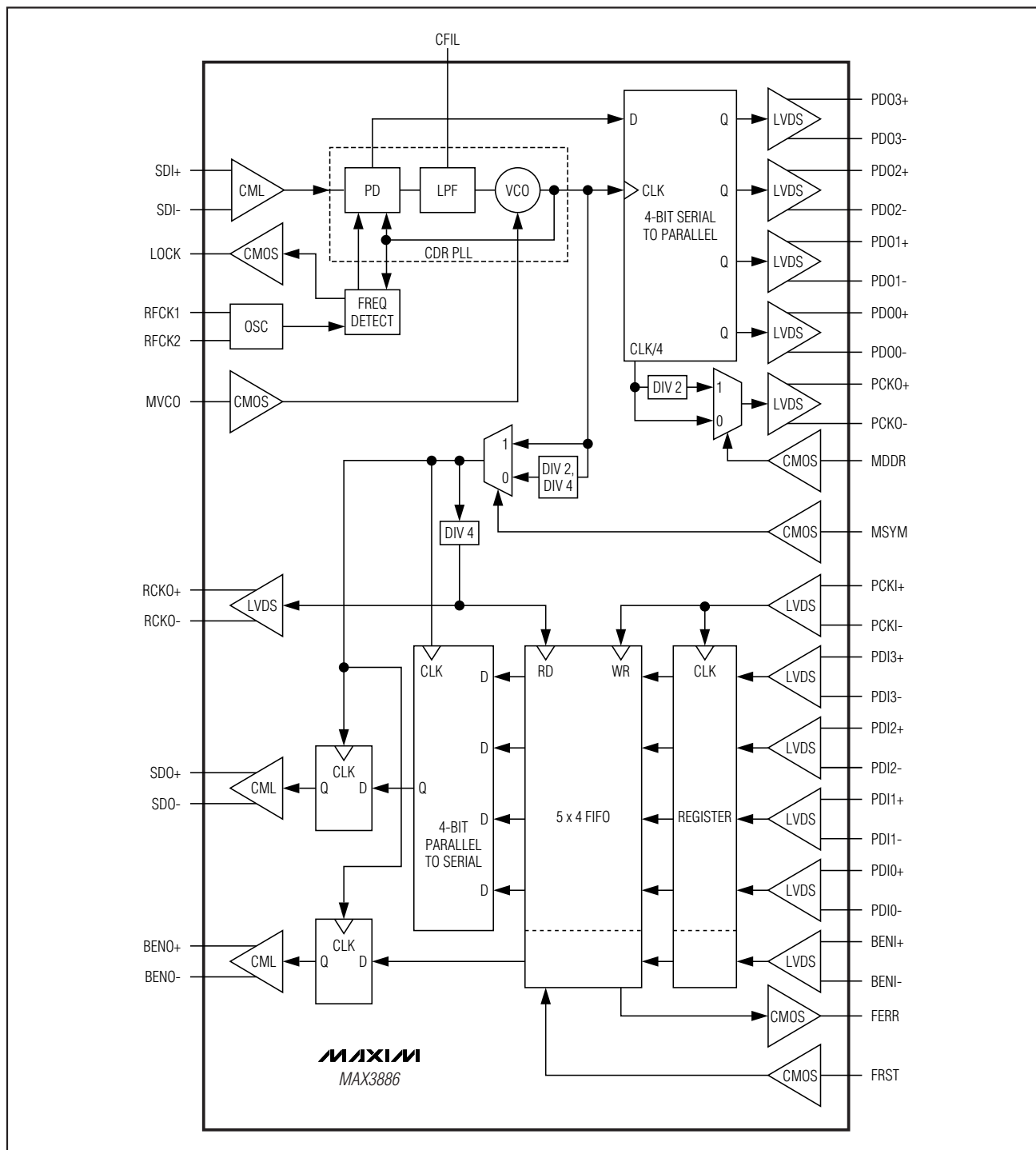
Figure 4. Functional Diagram
