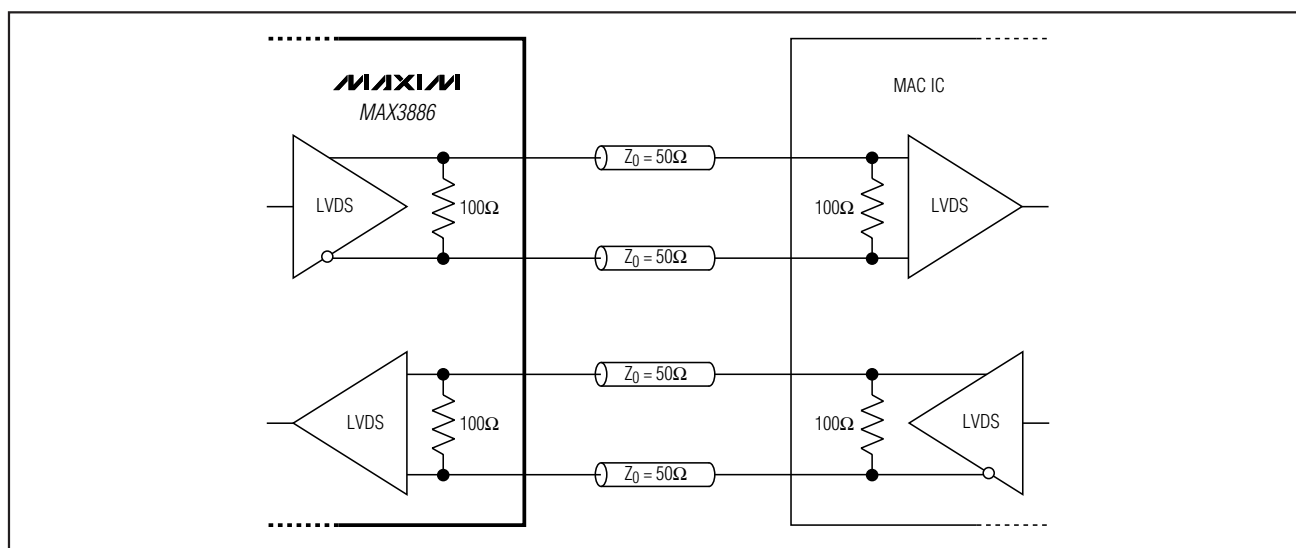
Figure 10. LVDS Interface
