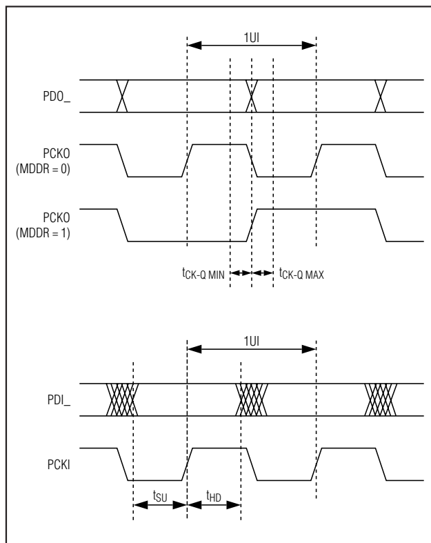
Figure 1. Parallel Interface Timing Diagrams
