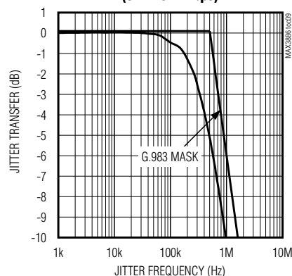
SDI TO SDO JITTER TRANSFER (SDI = 622Mbps)
