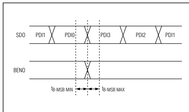
Figure 2. Burst-Enable Timing
