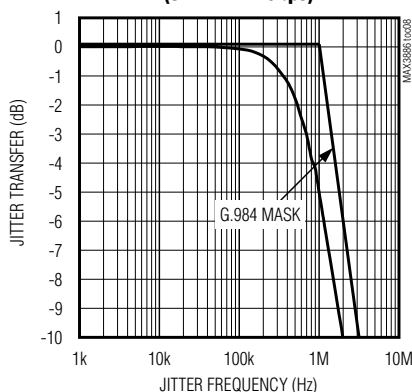
SDI TO SDO JITTER TRANSFER (SDI = 1.244Gbps)
