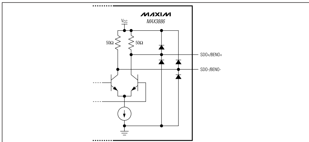
Figure 8. CML Outputs
