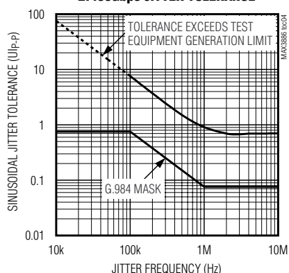
2.488Gbps JITTER TOLERANCE
