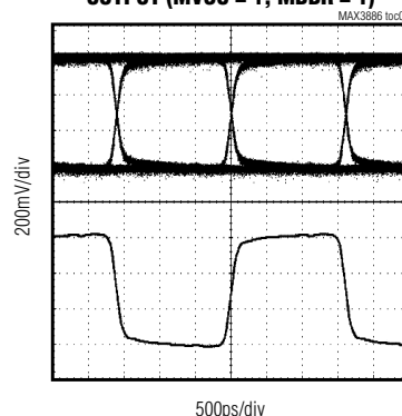
622Mbps PARALLEL DATA AND CLOCK OUTPUT (MVCO = 1, MDDR = 1)
