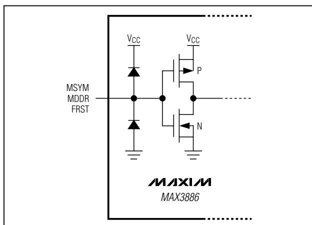
Figure 12. LVC MOS Inputs
