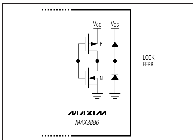
Figure 13. LVC MOS Outputs
