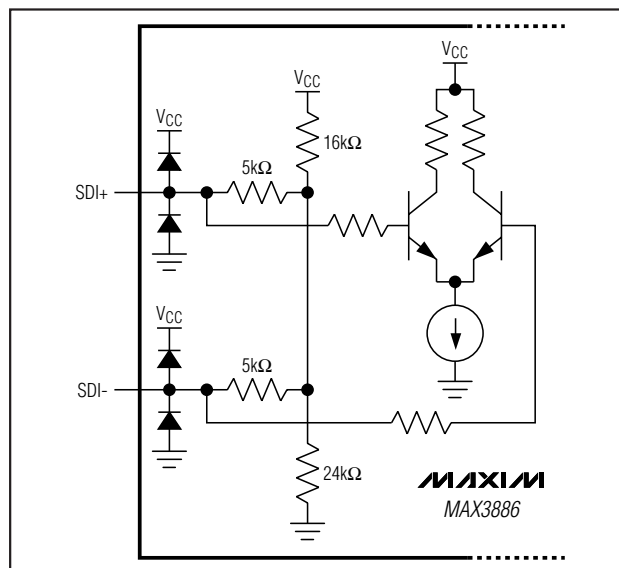
Figure 5. CML (LVPECL-Compatible) Input
