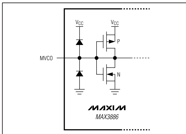
Figure 11. Three-State Input (MVCO)
