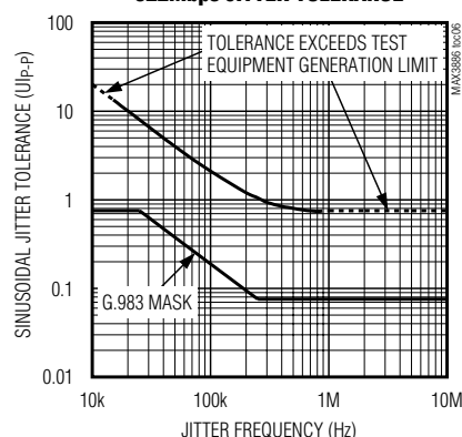
622Mbps JITTER TOLERANCE
