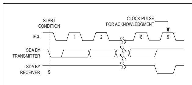
Figure 4. Acknowledge
