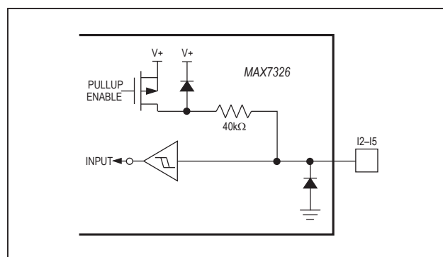
Figure 12. MAX7326 Input Port Structure
