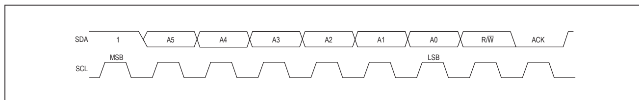
Figure 5. Slave Address
