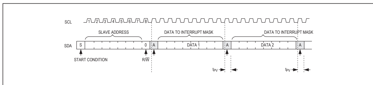
Figure 9. Writing to the Group A Ports of the MAX7326
