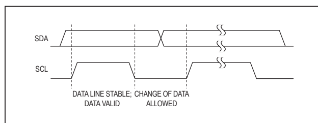
Figure 3. Bit Transfer
