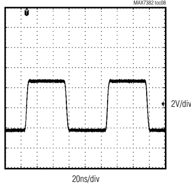
CLOCK OUTPUT WAVEFORM ( C_L = 10pF )
