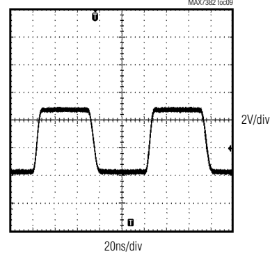
CLOCK OUTPUT WAVEFORM ( C_L = 10pF )
