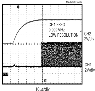
SETTLING TIME FROM START
