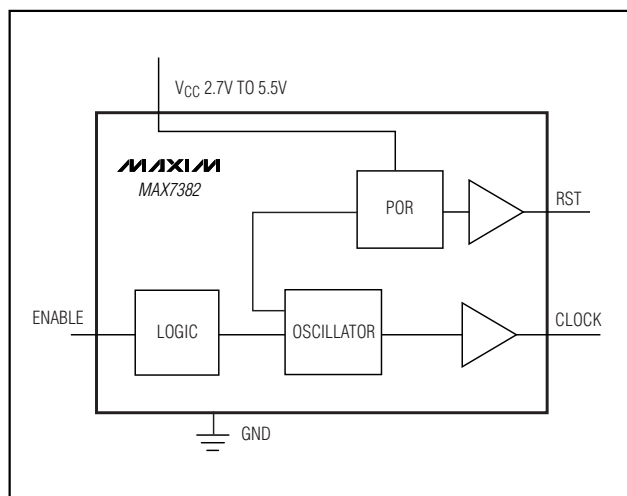
Figure 1. Functional Diagram
