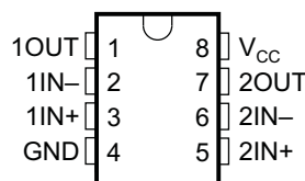
LM293 . . . D PACKAGE (TOP VIEW)
