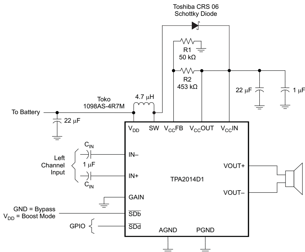
Figure 17. Bypass Circuit
