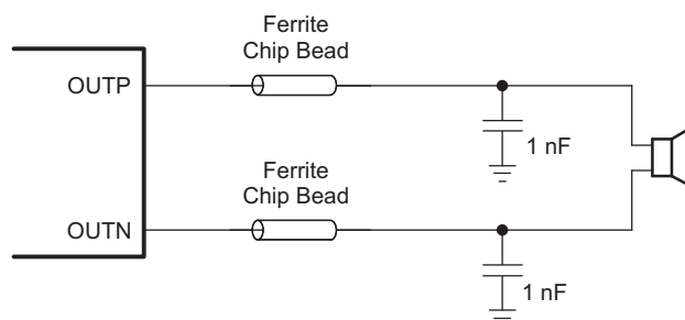
Figure 16. Typical Ferrite Chip Bead Filter
