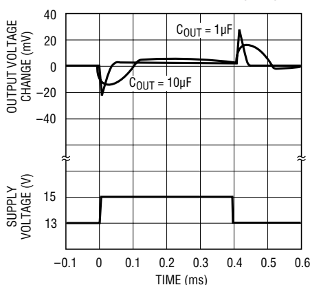
Line Transient Response (12V)
