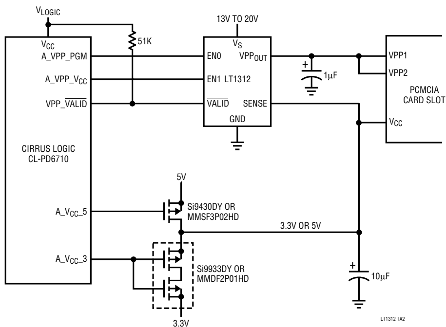
Single Slot Interface to CL-PD6710
