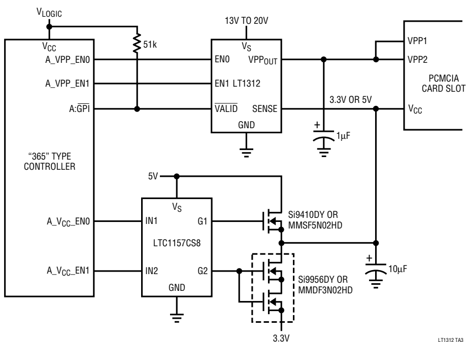
Single Slot Interface to "365" Type Controller
