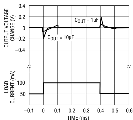
Load Transient Response (12V)
