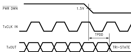
Figure 10. Transmitter Power Down Delay
