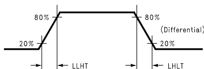
Figure 4. DS90CF383B (Transmitter) LVDS Transition Times
