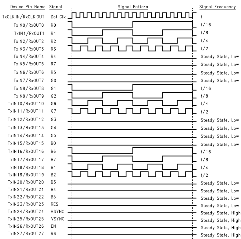
Figure 1. "Worst Case" Test Pattern
