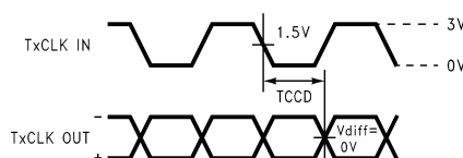
Figure 7. DS90CF383B (Transmitter) Clock In to Clock Out Delay (Falling Edge Strobe)
