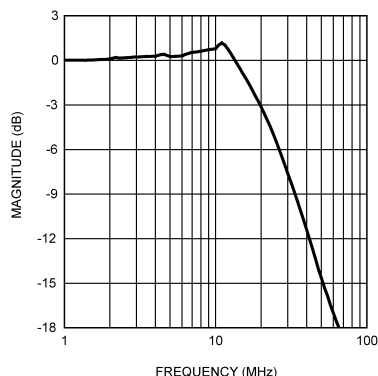
Figure 6. Bandwidth
