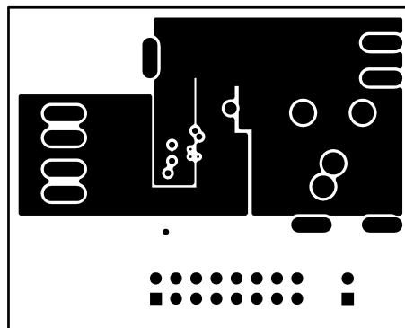
Figure 31. Layer 2 (GND)
