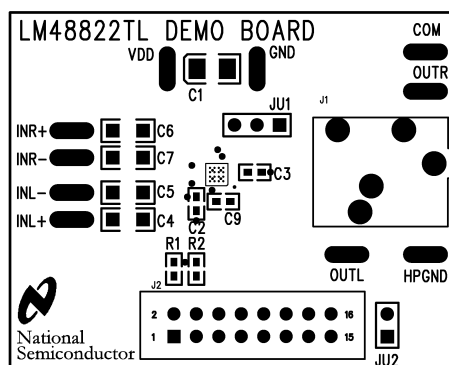
Figure 29. Top Silkscreen
