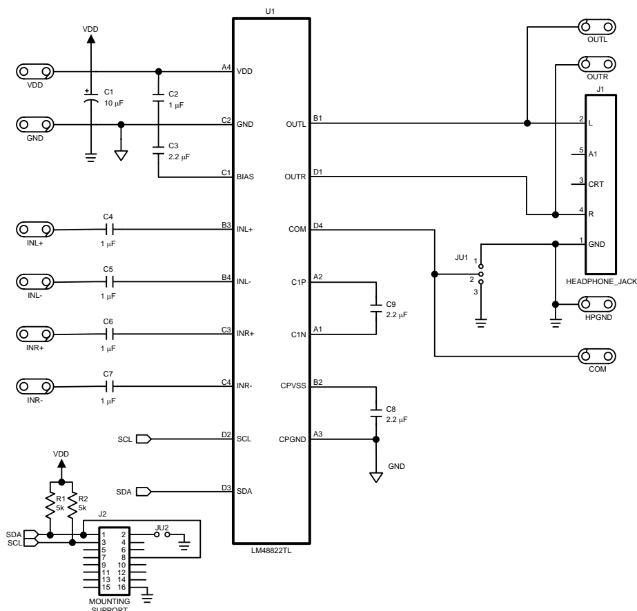
Figure 27. LM48822 Demoboard Schematic
