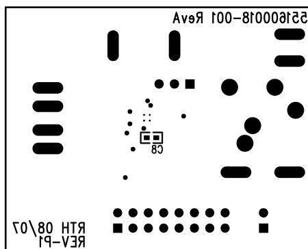
Figure 34. Bottom Silkscreen
