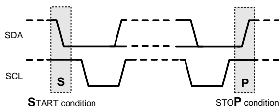
Figure 22. Start and Stop Diagram
