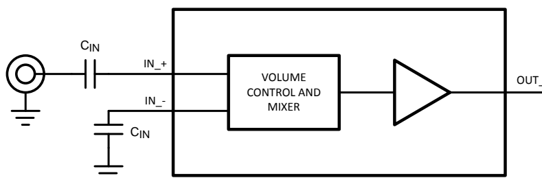
Figure 26. Single-Ended Input Configuration
