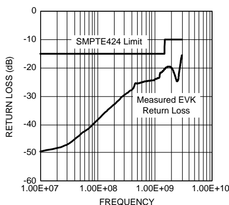
Figure 7. SDI Output Return Loss (EVK Example)
