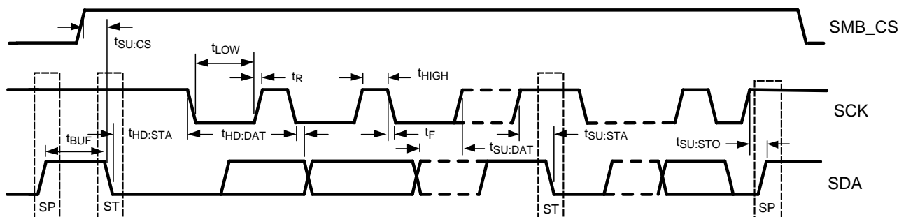
Figure 4. SMBus Timing Parameters
