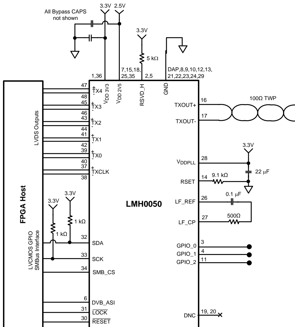
Figure 15. Typical LMH0050 CML Application Circuit
