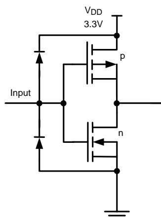
Figure 12. Simplified LVCMOS Input Circuit
