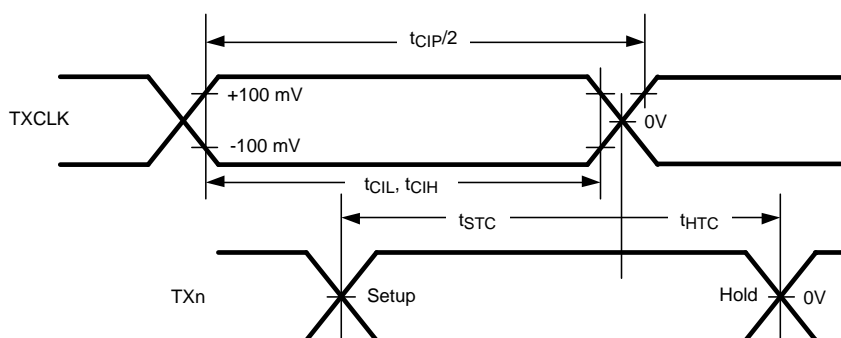
Figure 2. LVDS Input Timing Diagram
