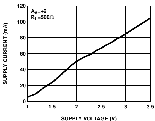
FIGURE 7. SUPPLY CURRENT vs SUPPLY VOLTAGE
