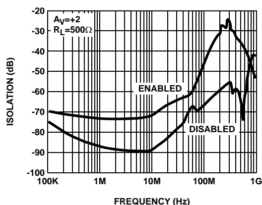
FIGURE 6. INPUT TO OUTPUT ISOLATION vs FREQUENCY
