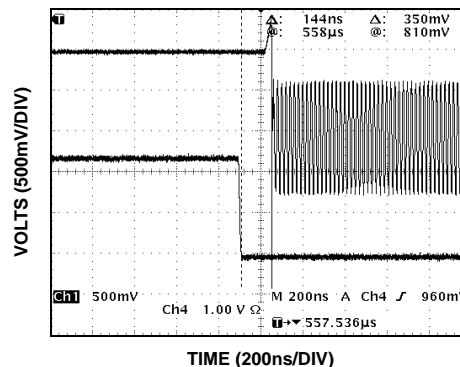
FIGURE 18. ENABLE TIME
