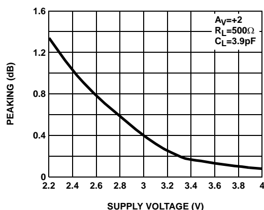
FIGURE 24. PEAKING vs SUPPLY VOLTAGE
