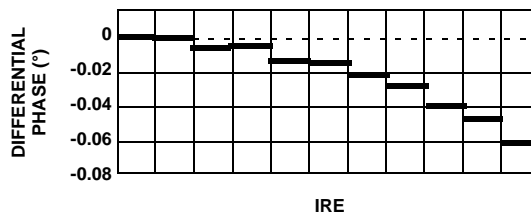
FIGURE 16. DIFFERENTIAL PHASE
