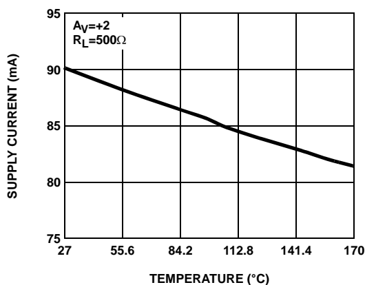
FIGURE 9. SUPPLY CURRENT vs TEMPERATURE
