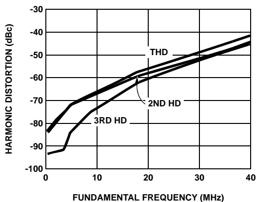
FIGURE 13. HARMONIC DISTORTION vs FREQUENCY
