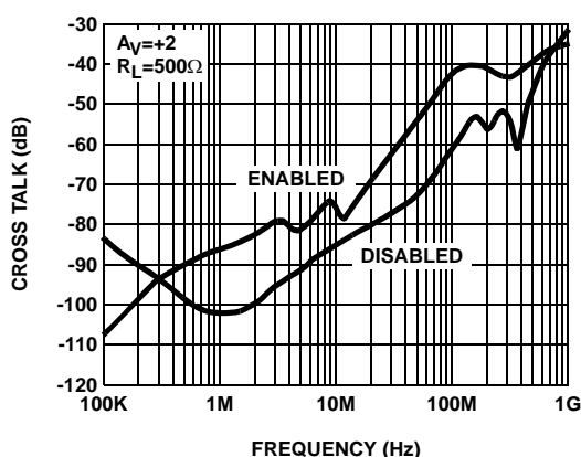
FIGURE 5. CROSS TALK CHANNEL TO CHANNEL (TYPICAL)
