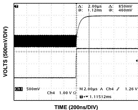
FIGURE 17. DISABLE TIME
