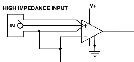
FIGURE 38. GUARD RING EXAMPLE FOR UNITY GAIN AMPLIFIER
