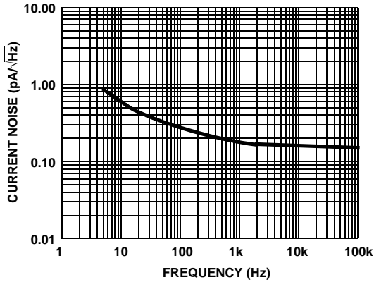
FIGURE 7. CURRENT NOISE vs FREQUENCY
