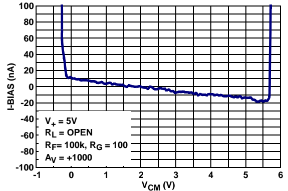
FIGURE 14. INPUT OFFSET CURRENT vs COMMON-MODE INPUT VOLTAGE
