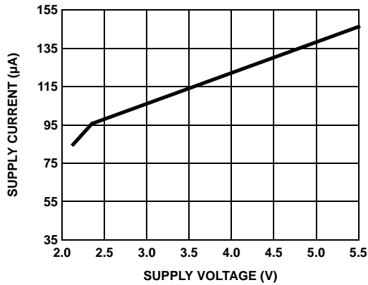
FIGURE 15. ISL28286 SUPPLY CURRENT vs SUPPLY VOLTAGE
