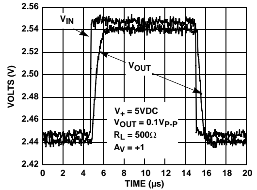
FIGURE 10. SMALL SIGNAL TRANSIENT RESPONSE
