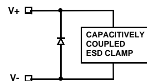
CIRCUIT 4
