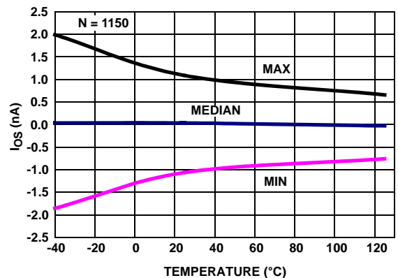
FIGURE 24. I_{OS} vs TEMPERATURE, V_+, V_- = \pm 2.5V
