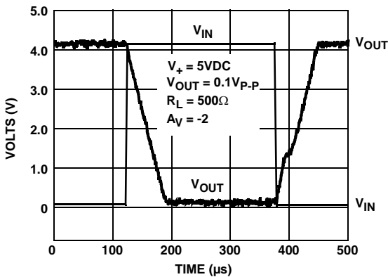
FIGURE 11. LARGE SIGNAL TRANSIENT RESPONSE
