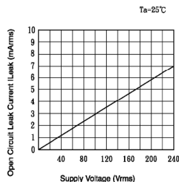
Fig.3 Open Circuit Leak Current vs. Supply Voltage
