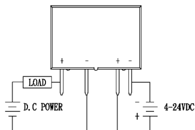
Fig.8 WIRING DIAGRAM
