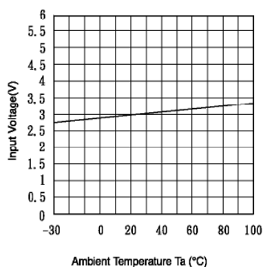
Fig.1 Input Voltage vs. Ambient Temperature
