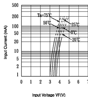
Fig.3 Input Current vs. Input Voltage
