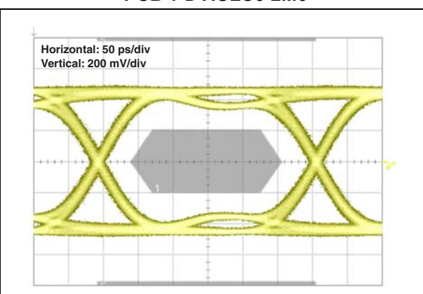
Figure 7. Eye diagram at 3.2 Gbps amplitude 500 mV PCB + DVIULC6-2M6
