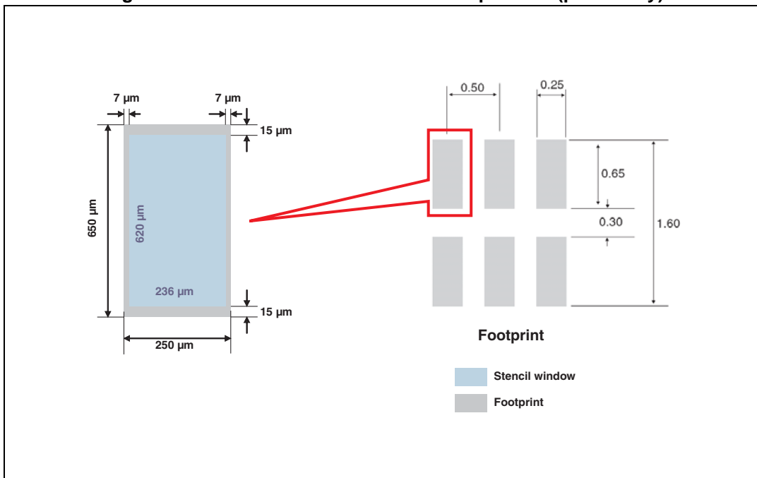
Figure 21. Recommended stencil window position ( \mu\text{QFN} only)
