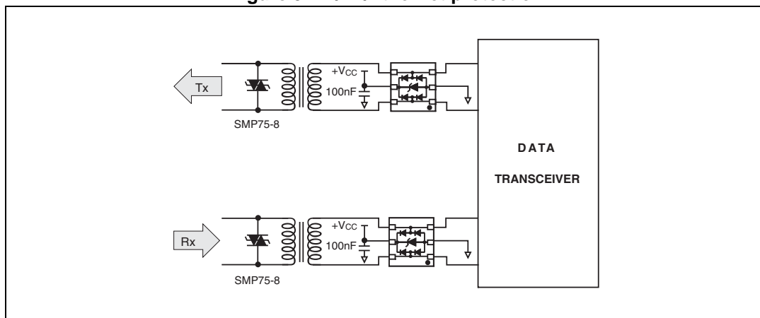
Figure 9. T1/E1/Ethernet protection
