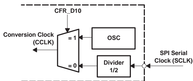
Figure 56. Converter Clock
