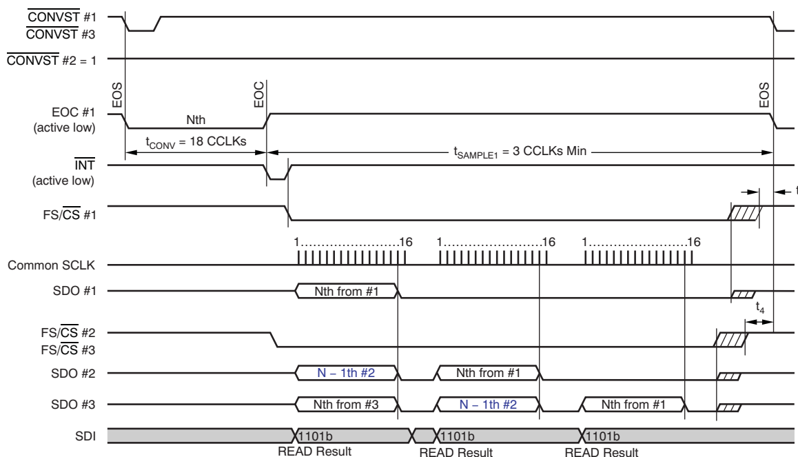
Figure 64. Simplified Cascade Timing (Separate \overline{\text{CONVST}} )
