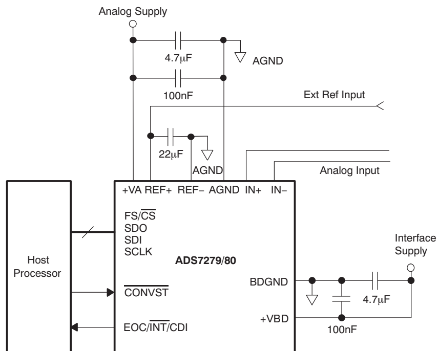
Figure 68. Typical Circuit Configuration
