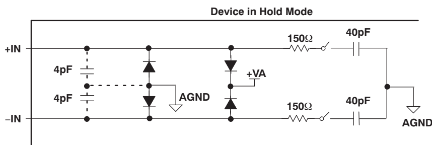
Figure 53. Input Equivalent Circuit
