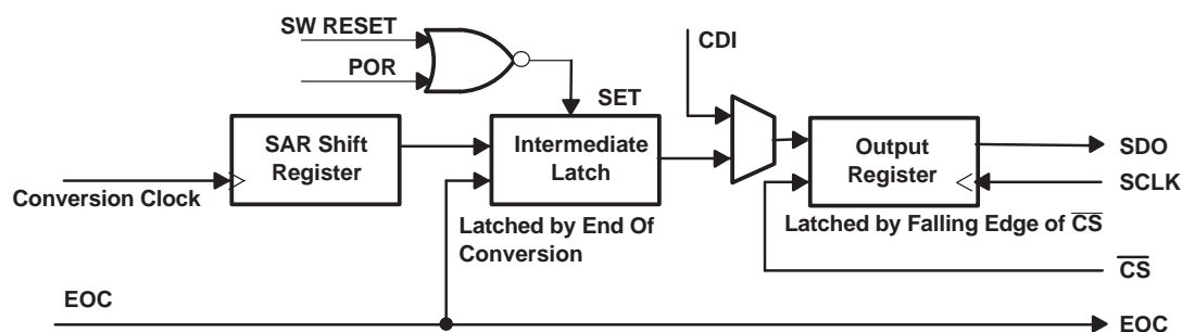
Figure 66. Digital Output Under Reset Condition
