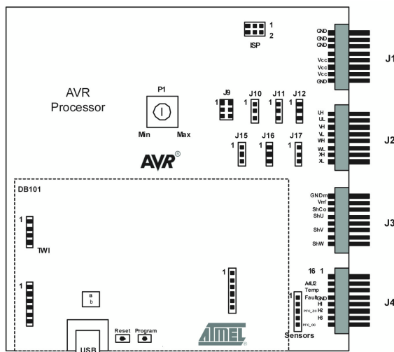
Figure 2-1. Processor board placement
