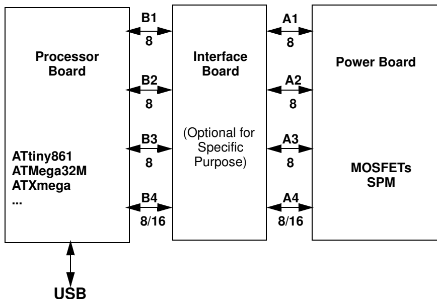
Figure 1-1. System Architecture
