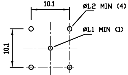
MOUNTING HOLE
