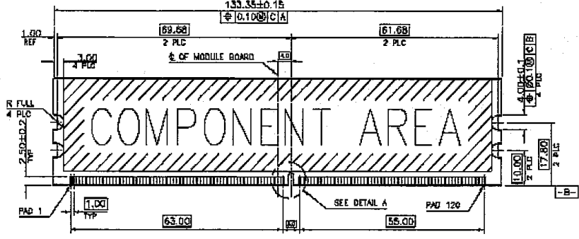
RECOMMENDED MODULE LAYOUT
