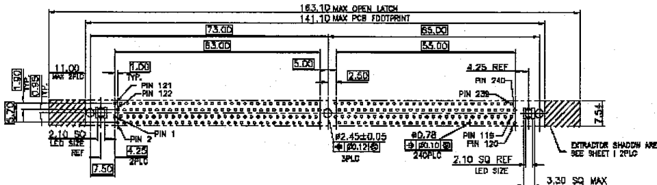
RECOMMENDED PCB LAYOUT PCB TOLERANCE: ±0.05
