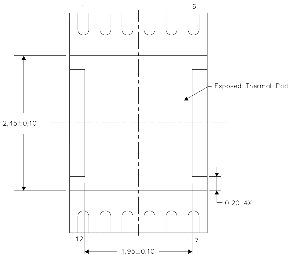
Bottom View
