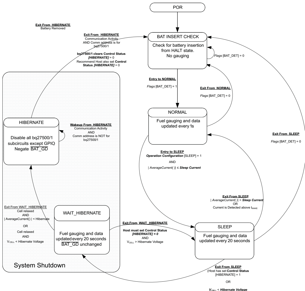
Figure 5-2. Power Mode Diagram
