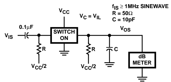
FIGURE 12. SWITCH OFF SIGNAL FEEDTHROUGH
