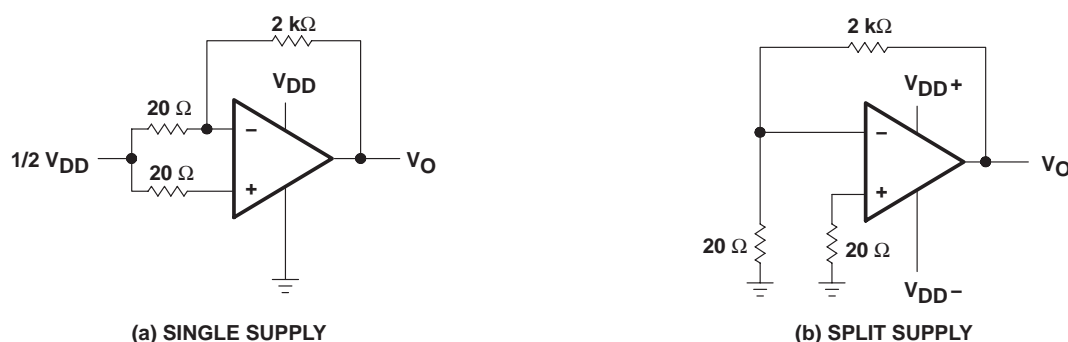
Figure 2. Noise-Test Circuit
