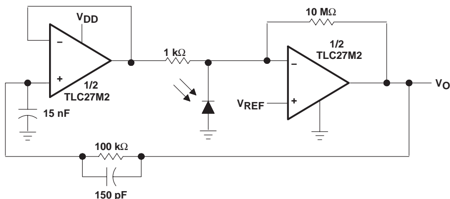
Figure 47. Photo-Diode Amplifier With Ambient Light Rejection
