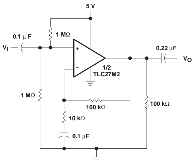
Figure 49. Single-Rail AC Amplifiers
