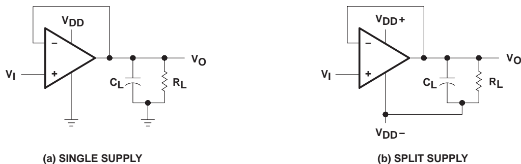
Figure 1. Unity-Gain Amplifier
