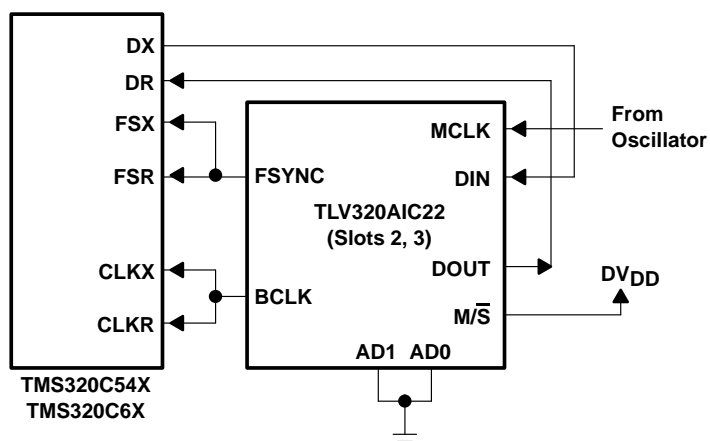
Figure 19. TLV320AIC22s Interface to McBSP Port of C54x or C6x DSP
