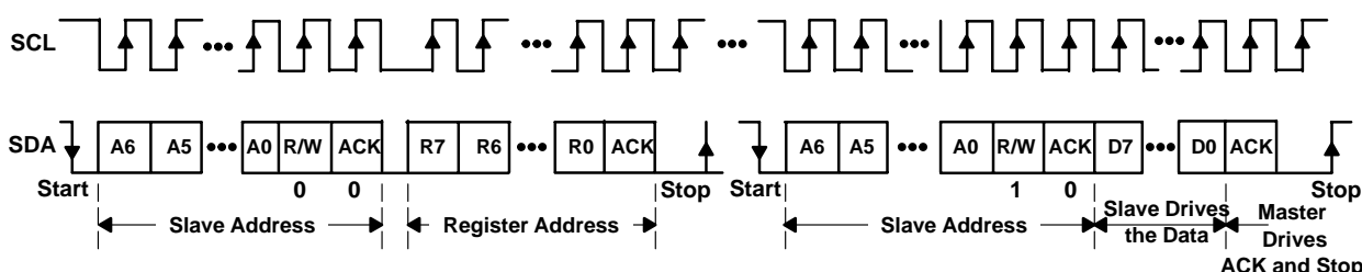
Figure 18. I 2 C Read From TLV320AIC22 (Protocol B)
