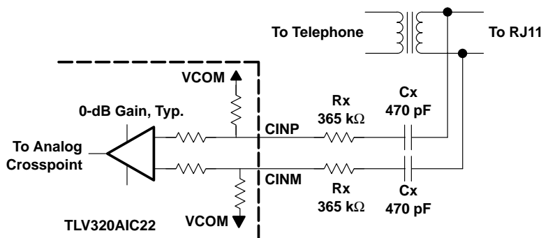
Figure 23. Typical Application Circuit for CallerID Amplifiers
