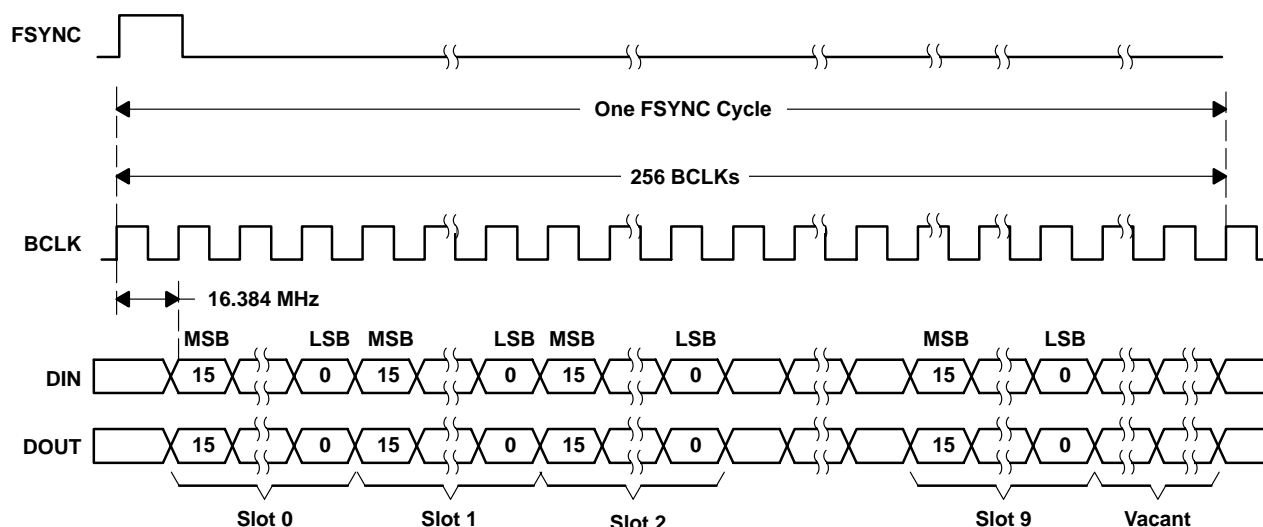
Figure 4. Timing Diagram for the TLV320AIC22 Frame Format
