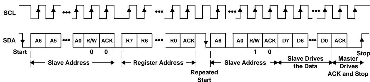
Figure 17. I 2 C Read From TLV320AIC22 (Protocol A)
