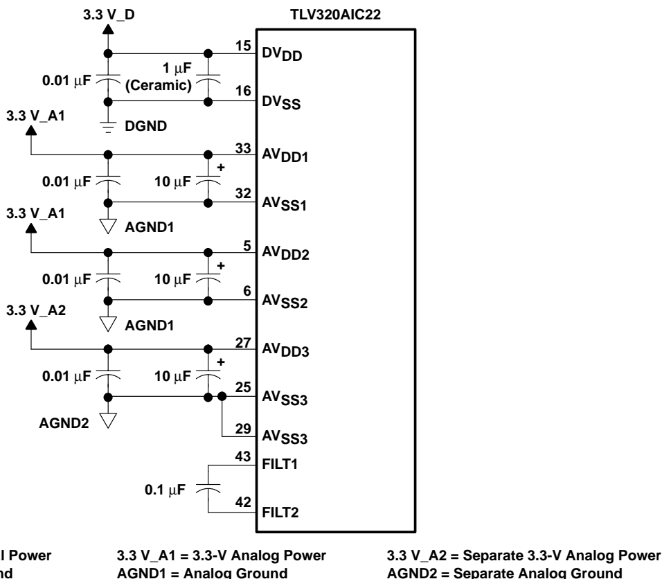
Figure 24. Recommended Decoupling
