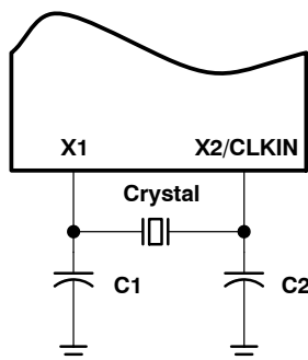
Figure 2. Internal Clock Option
