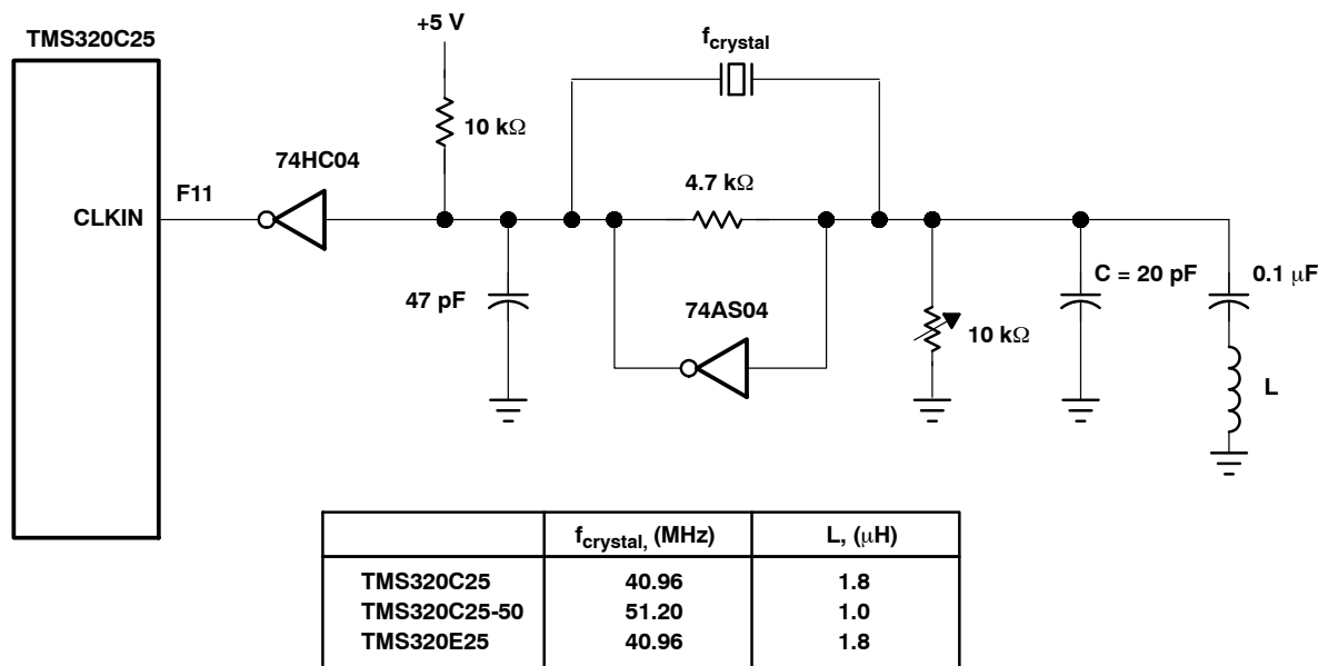
Figure 7. External Clock Option
