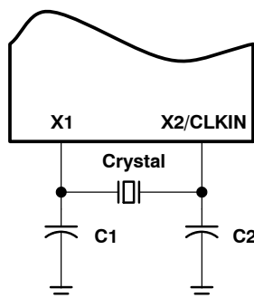
Figure 6. Internal Clock Option
