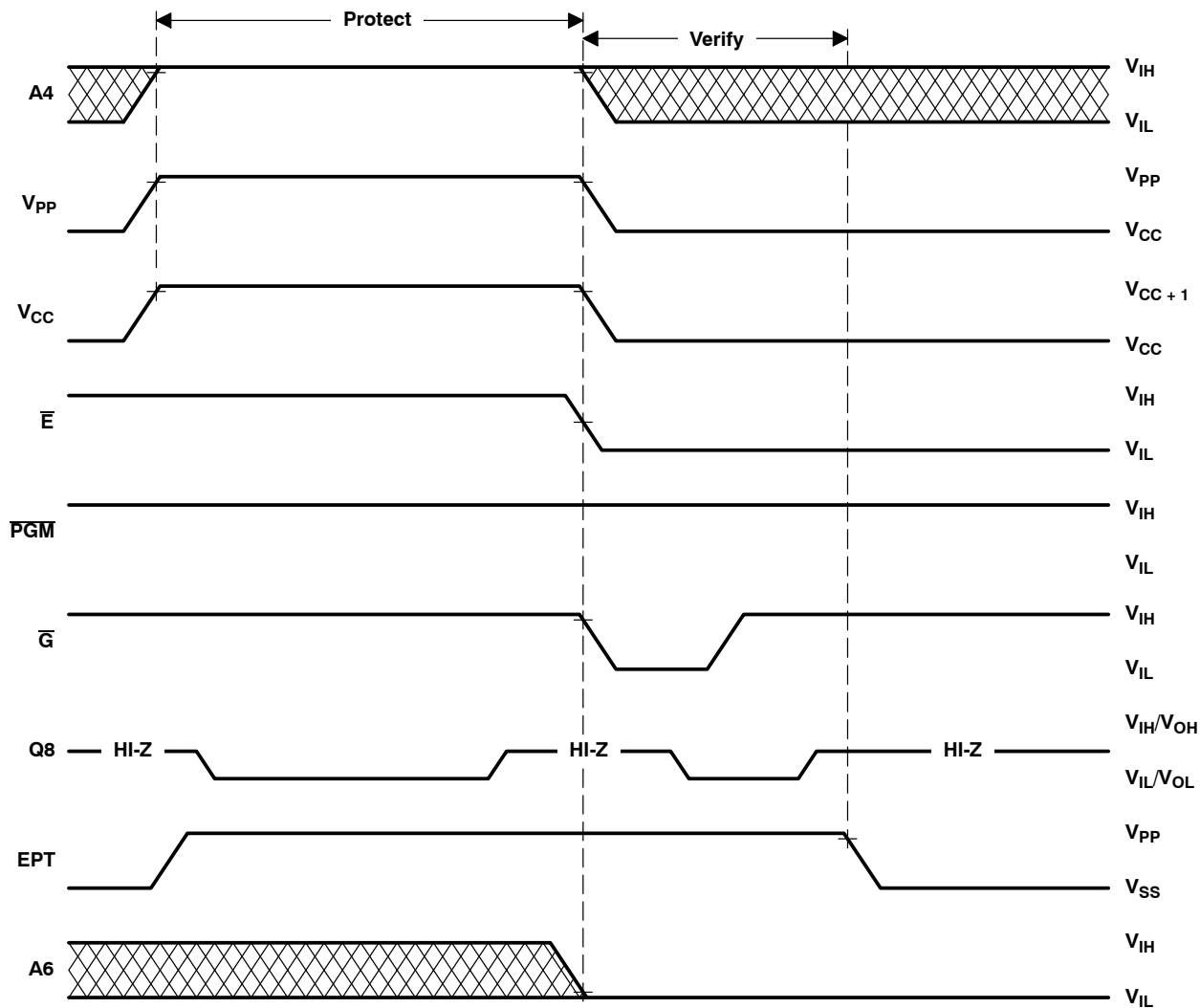
Figure 13. EPROM Protect Timing
