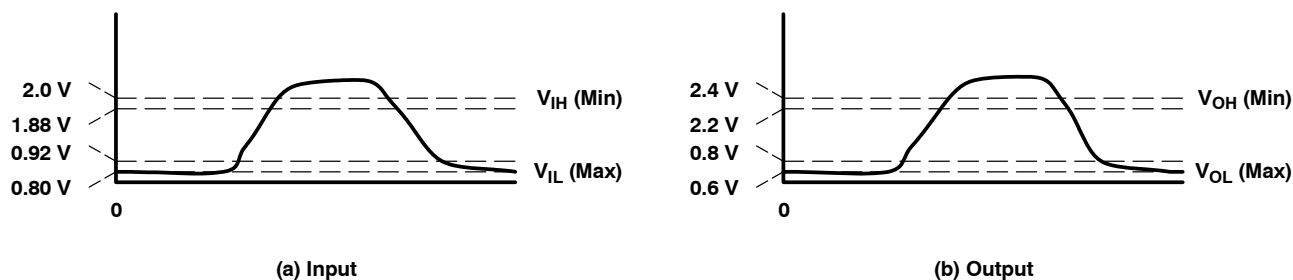
Figure 5. Voltage Reference Levels
