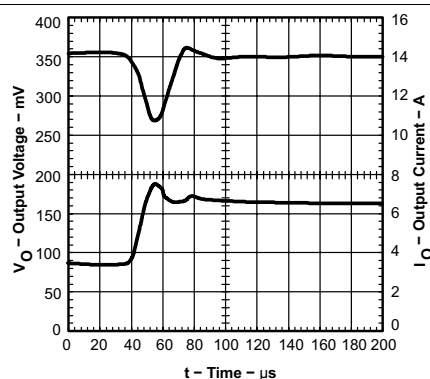
Figure 14. Transient Response
