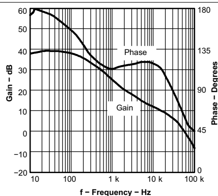
Figure 13. Loop Response
