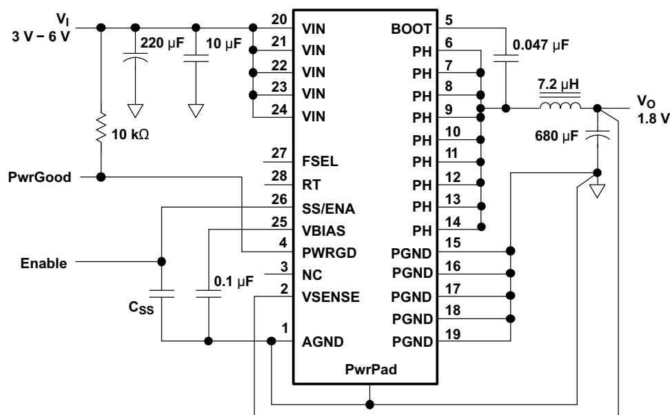
Figure 10. Application Circuit
