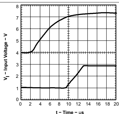
Figure 15. Start-up Waveforms
