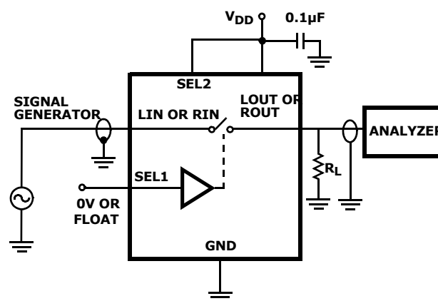
FIGURE 3. OFF ISOLATION CIRCUIT
