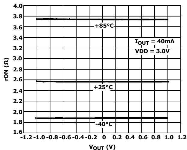
FIGURE 8. ON-RESISTANCE vs SWITCH VOLTAGE vs TEMPERATURE
