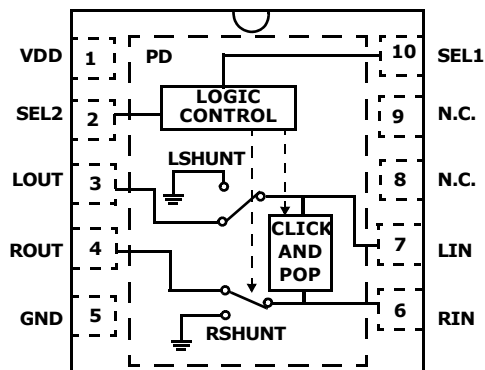
ISL54406 (10 Ld 3x3 TDFN) TOP VIEW
