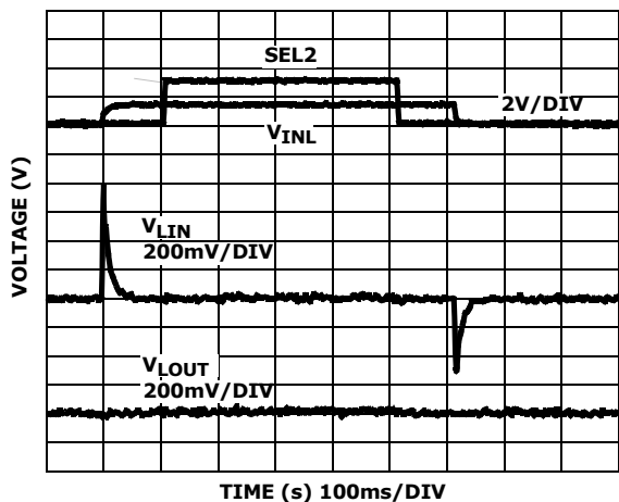
FIGURE 17. 20k \Omega CLICK AND POP REDUCTION
