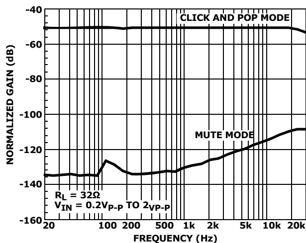
FIGURE 14. OFF-ISOLATION
