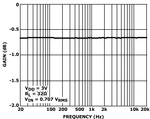
FIGURE 13. INSERTION LOSS
