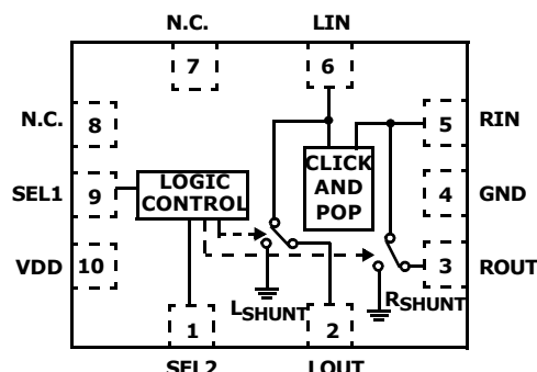
ISL54406 (10 Ld 1.8x1.4 \mu TQFN) TOP VIEW
