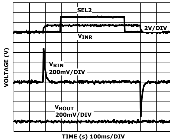
FIGURE 18. 32 \Omega CLICK AND POP REDUCTION
