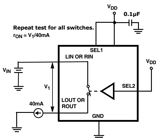
FIGURE 2. r_{ON} TEST CIRCUIT
