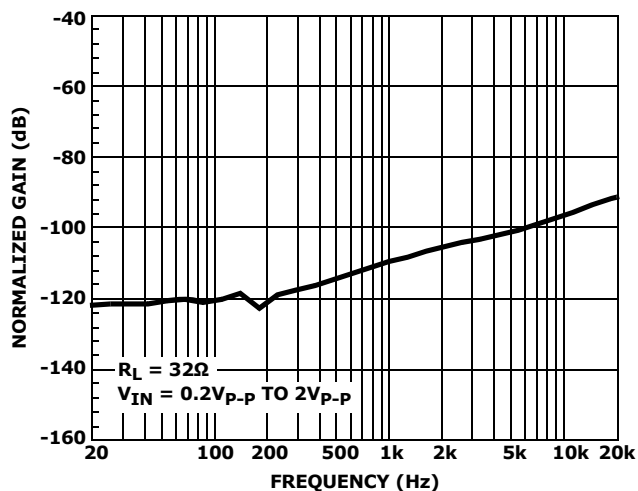
FIGURE 15. CROSSTALK
