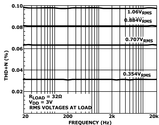
FIGURE 10. THD+N vs SIGNAL LEVELS vs FREQUENCY
