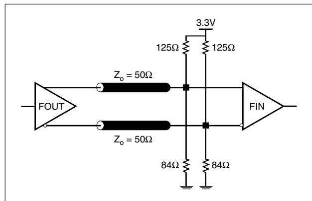
FIGURE 6B. LVPECL OUTPUT TERMINATION
