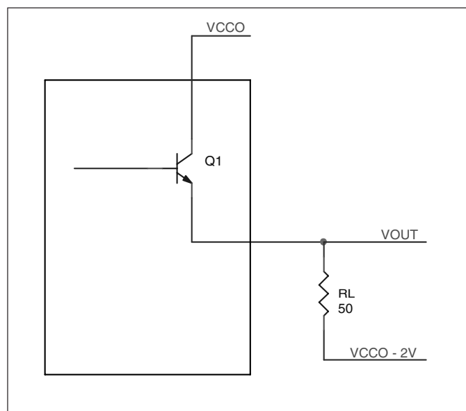
FIGURE 8. LVPECL DRIVER CIRCUIT AND TERMINATION
