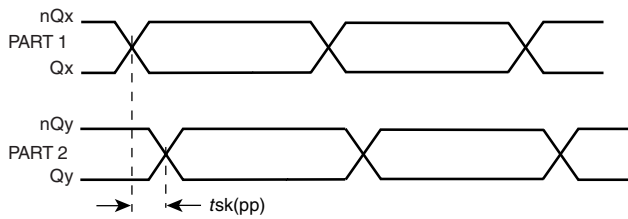
PART-TO-PART SKEW
