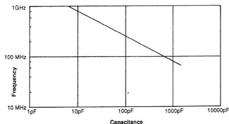
Self-Resonant Frequency vs. Capacitance
