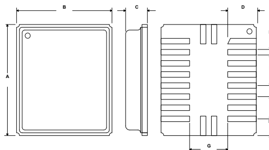
SM-20L Package Drawing
