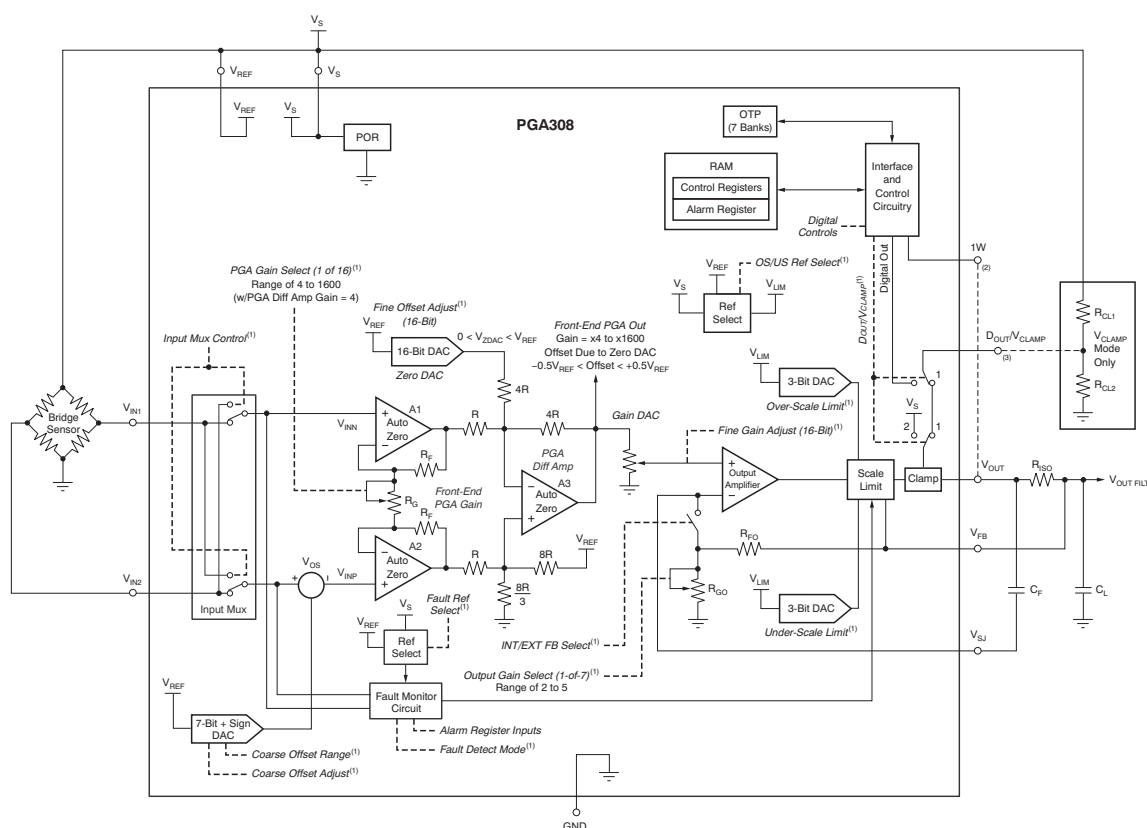
Figure 37. Detailed Block Diagram
