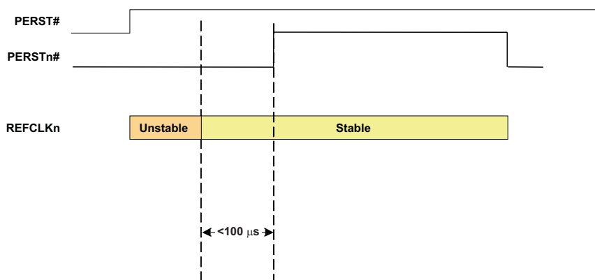
Figure 5-1. NonPCI Hot Plug Power-Up Cycle
