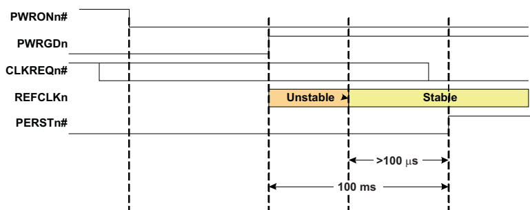
Figure 5-2. PCI Hot Plug Power-Up Cycle With PWRGDn Feedback
