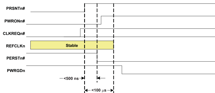
Figure 5-5. Surprise Removal
