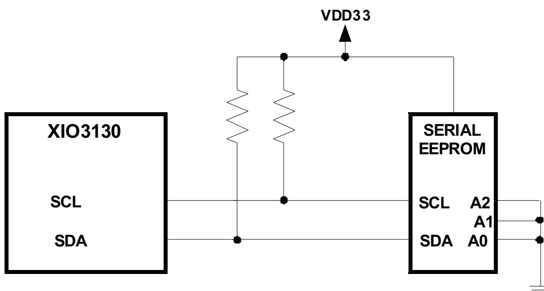
Figure 3-4. Serial EEPROM Applications
