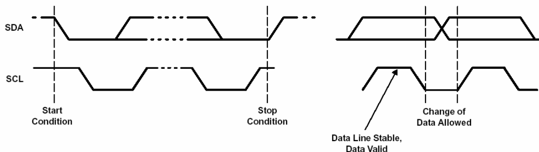
Figure 3-5. Serial-Bus Start/Stop Conditions and Bit Transfers
