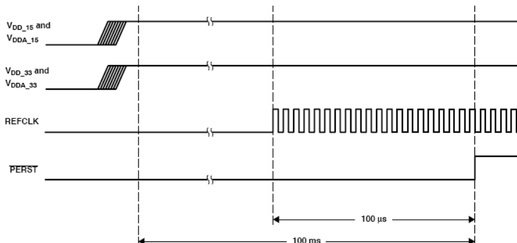
Figure 3-2. Power-Up Sequence Diagram
