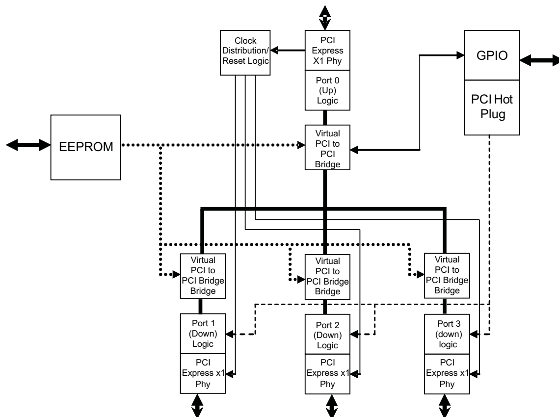
Figure 3-1. Block Diagram
