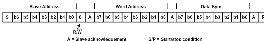
Figure 3-7. Serial-Bus Protocol – Byte Write
