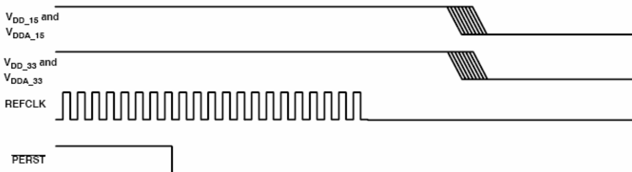
Figure 3-3. Power-Down Sequence Diagram
