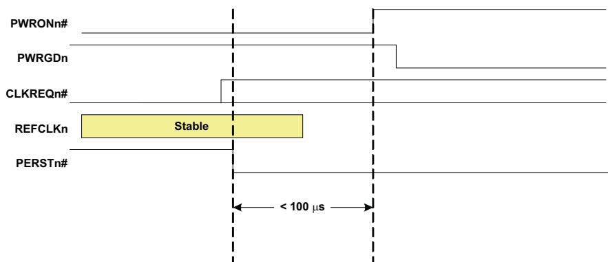
Figure 5-4. Normal Power-Down
