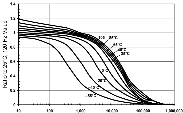
Capacitance vs. Temperature & Frequency
