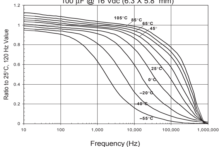
Capacitance vs. Temperature & Frequency
