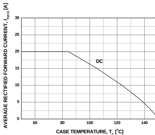
Figure 6. Forward Current Deration Curve
